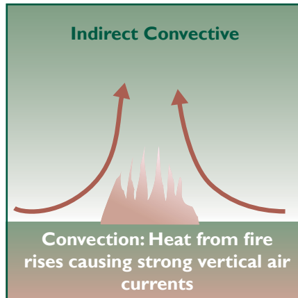
Convective lifting
